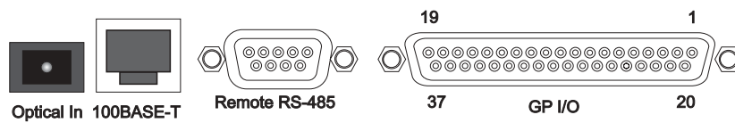
Figure 2-2 Connection Ports for Optical, Ethernet, Remote, and GPIO/O
